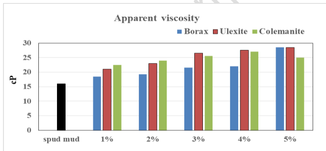
Figure 2 Apparent viscosities of the developed mud systems
