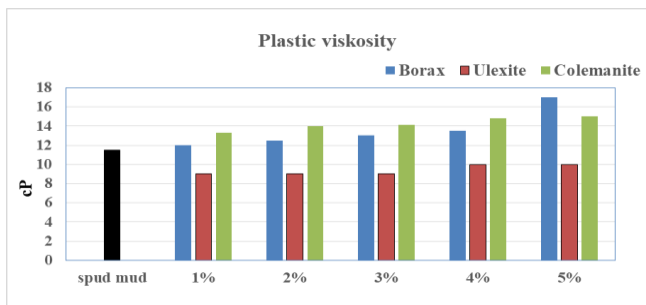
Figure 1: Plastic viscosities of the developed mud systems
