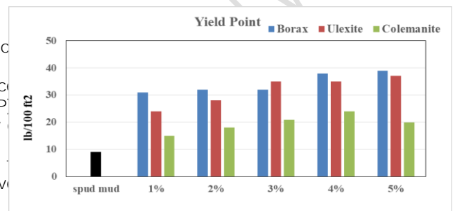
Figure 3 Yield points of the developed mud systems
