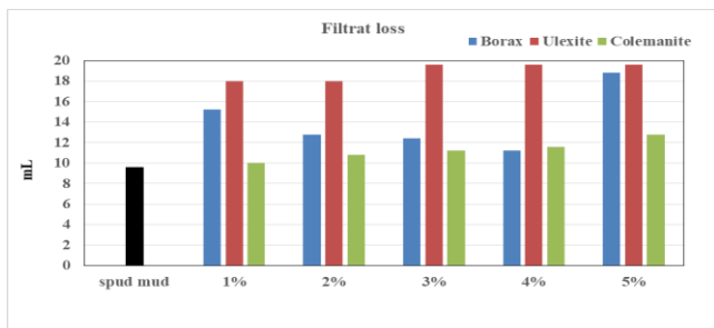
Figure 6: Filtrate loss of the developed mud systems
