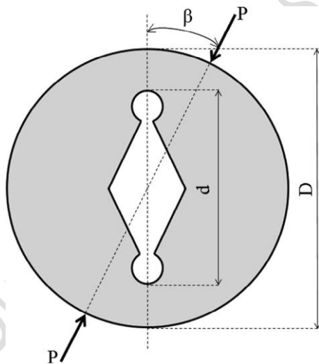
Figure 8: Brazilian disk specimen which has V-notches with end holes [26].
