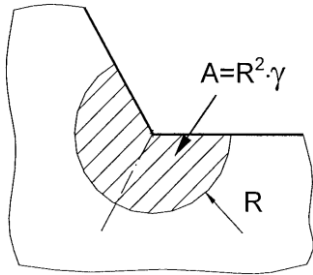
Figure1: Critical volume surrounding the notch tip [1].
