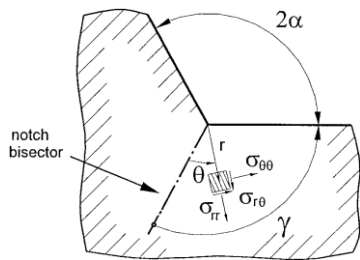
Figure2: Notch angles in polar coordinate system for notch tip [1].
