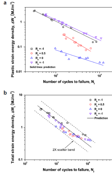
Figure 5: Fatigue life estimations based on (a) plastic SED, and (b) total SED [8].
