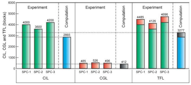
Figure 6: Comparison of experimental and computational results of crack initial, crack growth life and total fatigue life [14].
