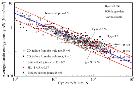
Figure 4: Fatigue strength of welds as a function of the averaged local SED [5].
