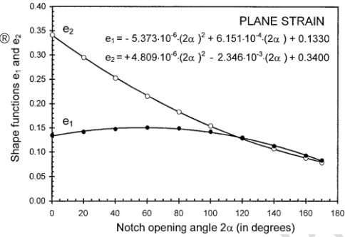
Figure3: Plot of total strain energy coefficients against the notch opening angle [1].
