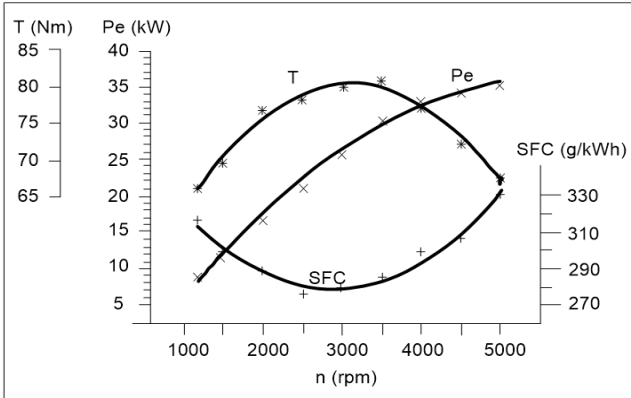
Figure 2: Characteristics of the test engine.
