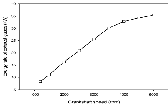
Figure 8: Variation of exergy rate associated with work with crankshaft speed.
