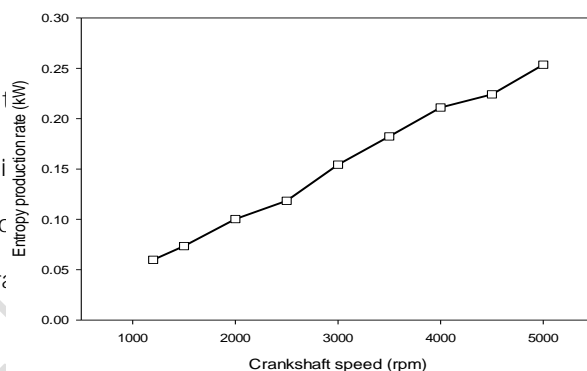
Figure 10: Variation of entropy production rate with crankshaft speed.
