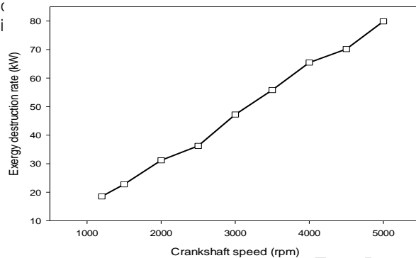
Figure 9: Variation of exergy destruction rate with crankshaft speed.
