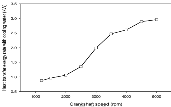
Figure 4: Variation of exergy rate associated with heat removed from the test engine through cooling water with crankshaft speed.
