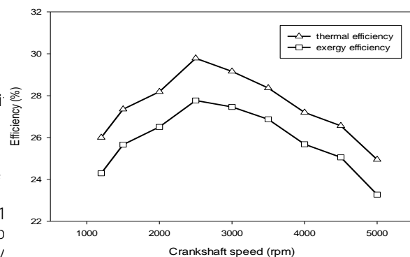
Figure 11: Variation of energy and exergy efficiencies with crankshaft speed.
