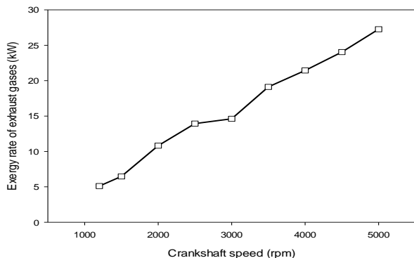
Figure 7: Variation of exergy rate of exhaust gases with crankshaft speed.
