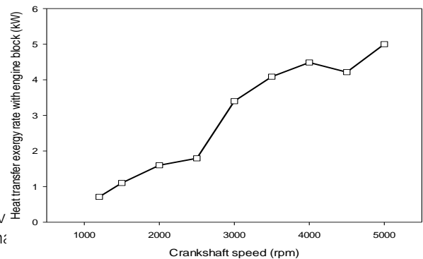
Figure 6: Variation of exergy rate associated with heat transferred from the engine block to environment with crankshaft speed.
