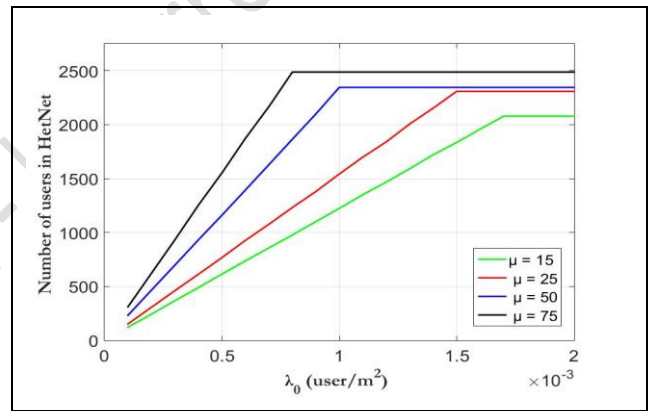
Figure3: Variation of the number of users in the HetNet for user density of the MBS.
