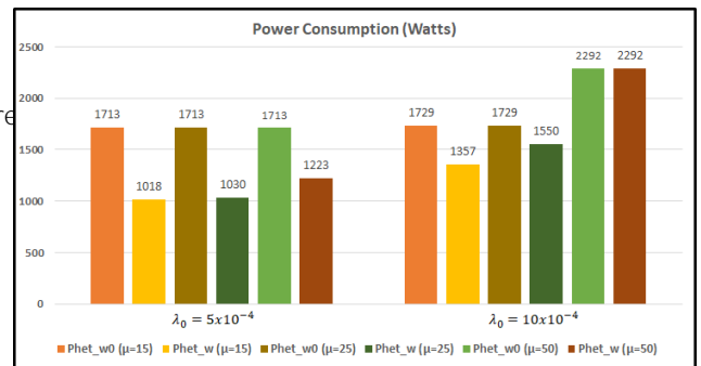
Figure 6: Power consumption of the HetNet with the MC user density ((w/o) and (with) mean that when the proposed algorithm is not used and used).
