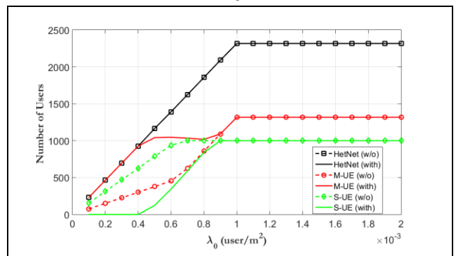
Figure4: Variation of the number of users in a HetNet where the proposed algorithm is used and not used. (w/o) in the MC, SUE: UE in the SCs, HetNet: UE in the HetNet, (w/o) and (with) mean that when the proposed algorithm is not used and used ( ).
