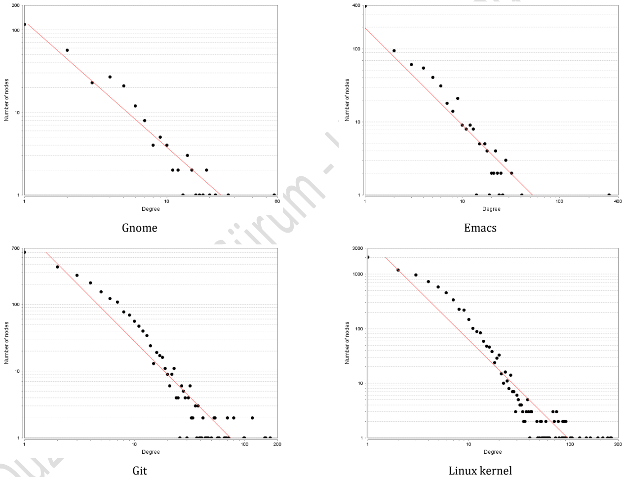
Figure 2: Degree distribution charts of the call graphs
