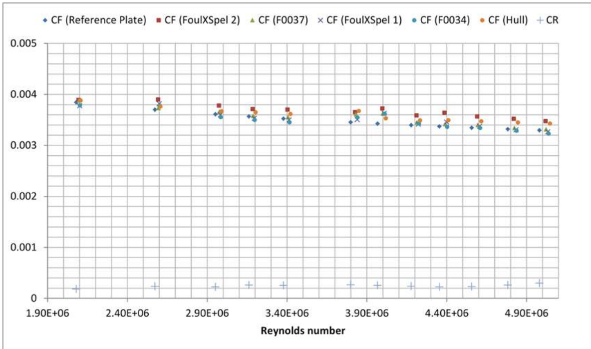
Fig. 4. Frictional resistance coefficients of all test surfaces together with CR values (Demirel et al., 2015)
