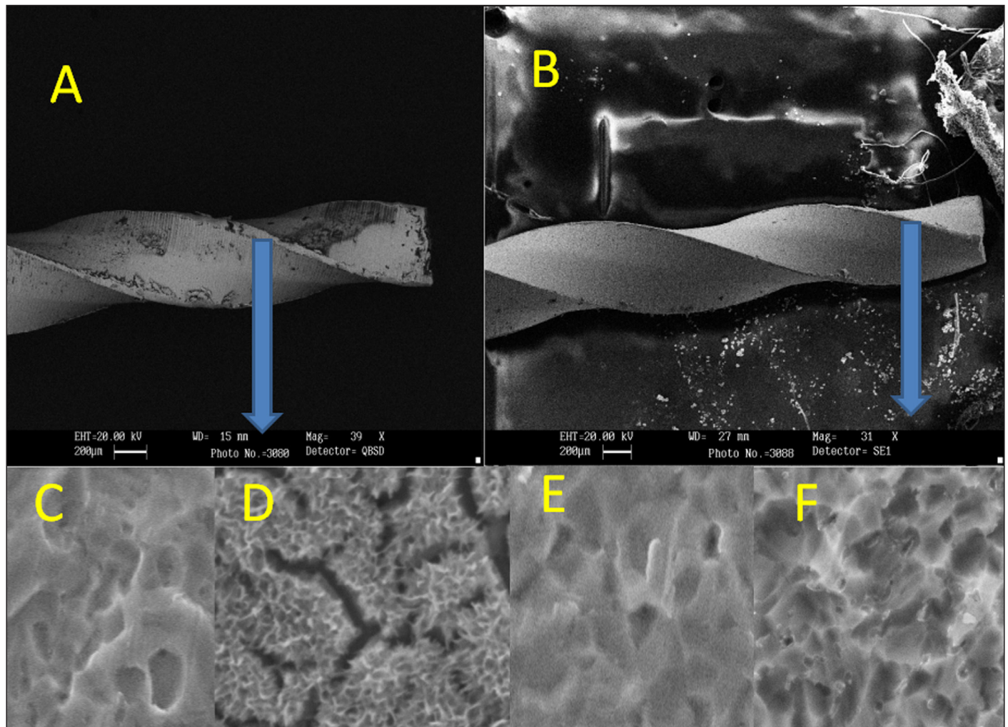
Figure 2. SEM micrographs for samples immersed in blood (39× mag) (A); SEM images of samples immersed in MOPA solution (31× mag) (B); SEM images of deionised water group showing irregular honeycomb pattern (2000× mag) (C); SEM images of blood group with intergranular pattern (2000× mag) (D); SEM images of PBS samples with macro dimple pattern (2000× mag) (E); SEM images of MOPA group specimens revealed honeycomb pattern with lesser impurities on the surface (2000× mag) (F). Please note that the arrows in A and B show the cutting edge of NiTi instruments that were used for further evaluation by 2000× magnification.
